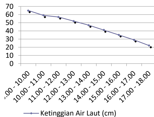
Figure 17. The Height Of The Tide In The Village Tallo.
