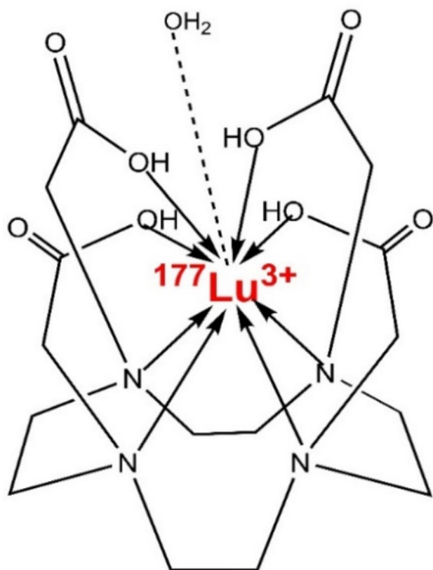
Fig. 2 Representative chemical structure of the [^{177}\text{Lu}]\text{Lu-DOTA} complex
