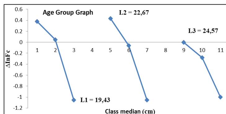
Fig 4: Graph of the difference between the natural logarithm of theoretical frequencies and the class median for male fish in each age group of Shortfin Scad ( Decapterus macrosoma ) in the waters of Bulukumba Regency.
