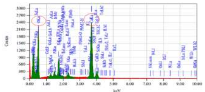
Figure 6. Qualitative Data of Point 1 test panel samplesased on the results of Energy Dispersive X- analysis
