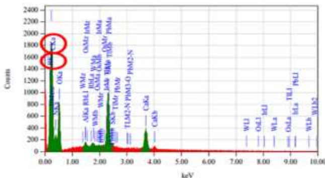
Figure 11. Qualitative data for point 2 test panel samples based on the results of Energy Dispersive X-ray analysis
