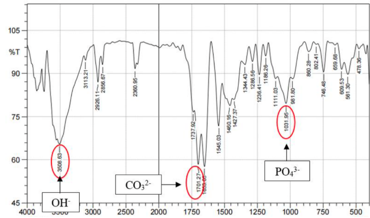
Figure 2. FTIR view of hydroxyapatite of bovine bone
