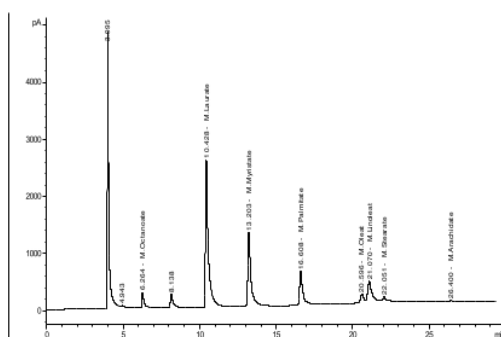
Figure 7. Chromatogram of Biodiesel product analysis Gas Chromatography
