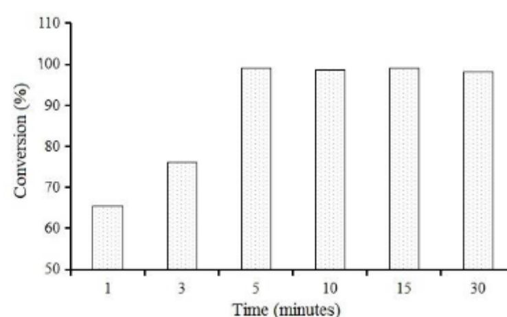
Figure 4. Effect of reaction time on the yield of the at NaOH 0.5% (w/w) concentration at 400 watt
