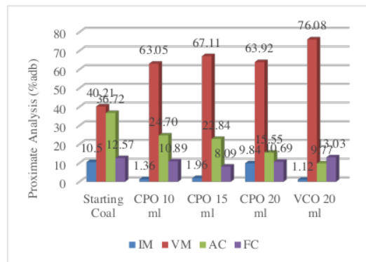
Figure 3. Comparison of proximate analysis after agglomeration process
