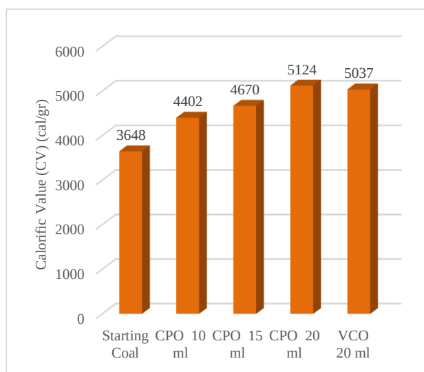
Figure 3. Calorific value (CV) comparison after agglomeration
