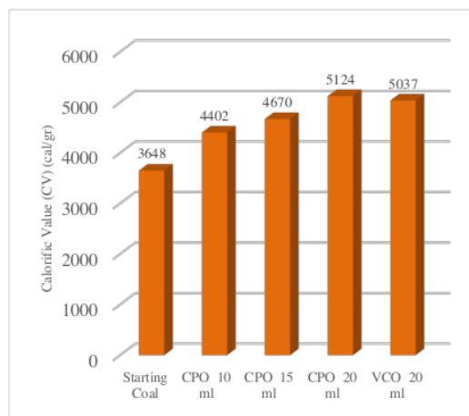
Figure 5. Calorific value (CV) comparison after agglomeration
