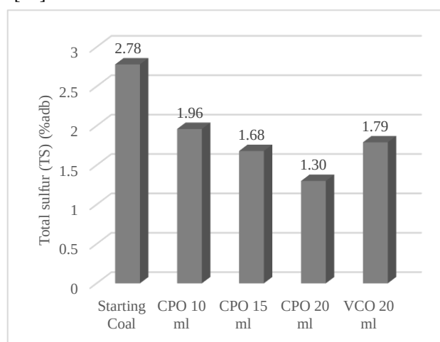
Figure 2. Comparison of total sulfur (S) after agglomeration process
