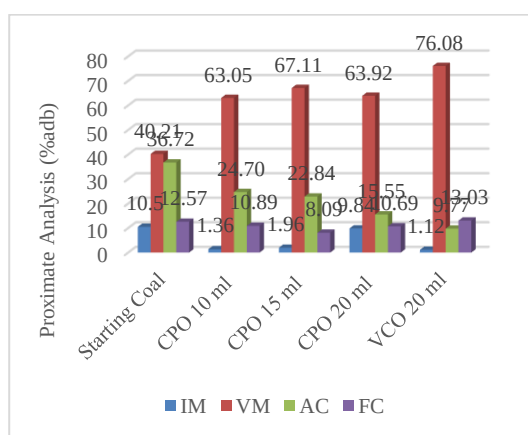
Figure 1. Comparison of proximate analysis after agglomeration process
