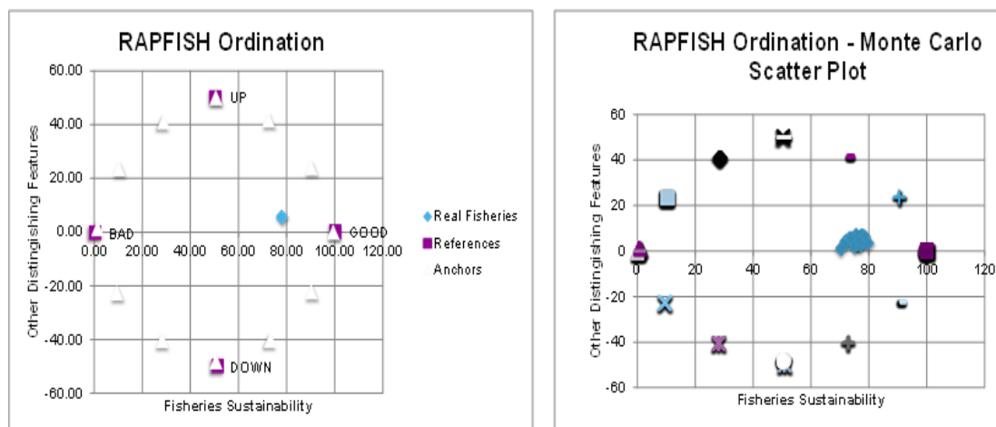
Fig. 2. Results of the ecological dimension ordination analysis
