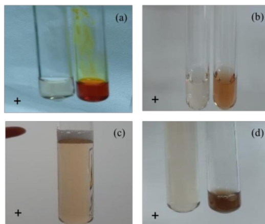
Fig. 1. Phytochemical analysis conducted on the epidermal extract of P. jiringa .
