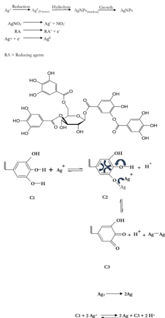
Fig. 5. Mechanism interaction between metal ions ( \text{Ag}^+ ) and reducing agents of tannin formation of AgNPs.
