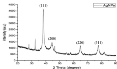
Fig. 9. XRD pattern analysis of P-jiringa-AgNPs.
