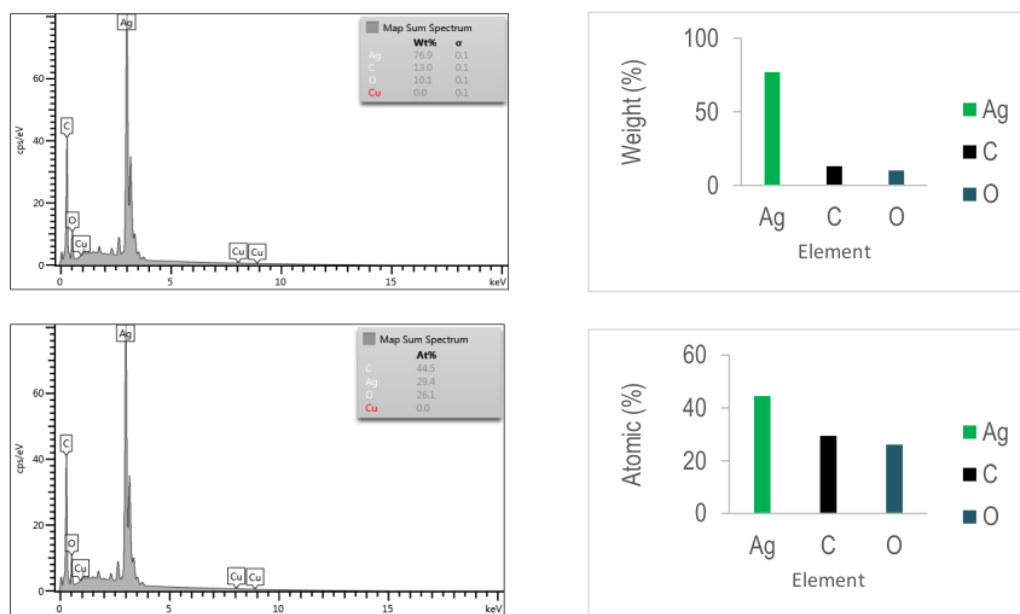
Fig. 8. Qualitative analysis of EDX elements (a) weight; (b) empirical atomic.
