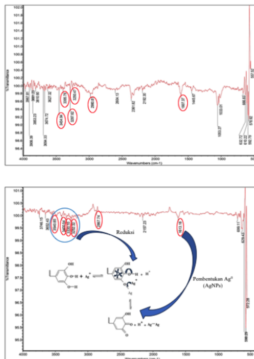
Fig. 6. Spectrum FTIR analysis of (a) P. jiringa epidermis extract, (b) AgNPs.
