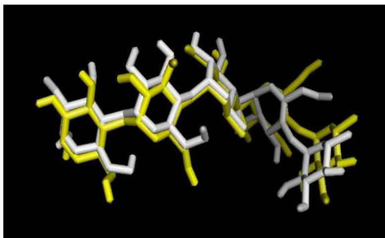
FIGURE 1. Overlay of the ligand position of the rootbosc redocking result with the crystallographic ligand (Yellow = Crystallographic result; White = Redcking result)
