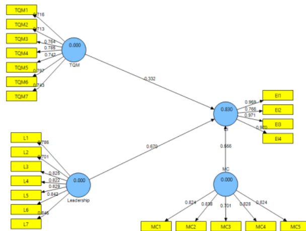
FIGURE 2 CONVERGENT VALIDITY, DISCRIMINANT, & DISCRIMINANT RELIABILITY TESTING
