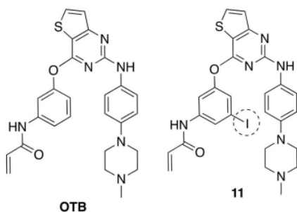
Fig 1. Structural formula of OTB and 11.
