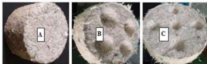
Figure 1 Specimen: A. Flat Surface (FS); B. 4 Concaves Surface (CS4); C. 5 Concaves Surface (CS5)
