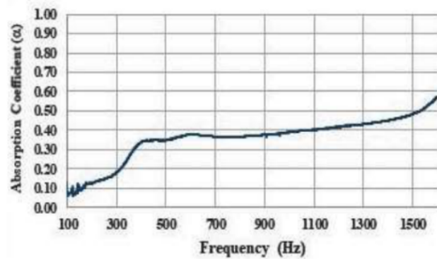
Figure 9 Average absorption coefficients of 4 Concave surface (CS4) specimen
