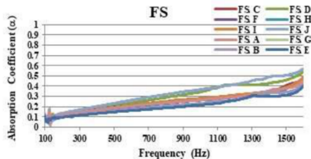
Figure 5. Absorption Coefficient of FS (A-J) samples
