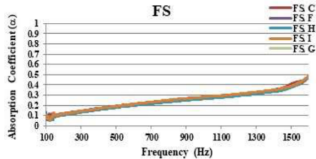
Figure 6. FS Absorption Coefficient Curve (C-F-H-I-G) sample
