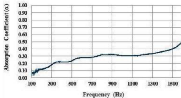
Figure 11. Graph of average \alpha for 5 Concave surface (CS5) specimen
