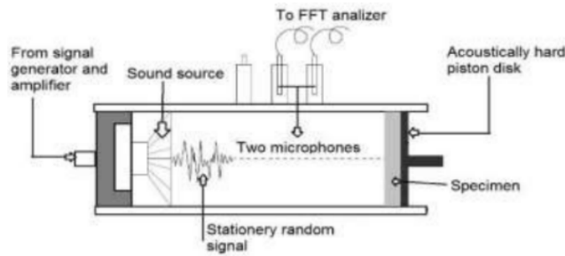
Figure 4. Schematic diagram of the two microphone of Impedance Tube
