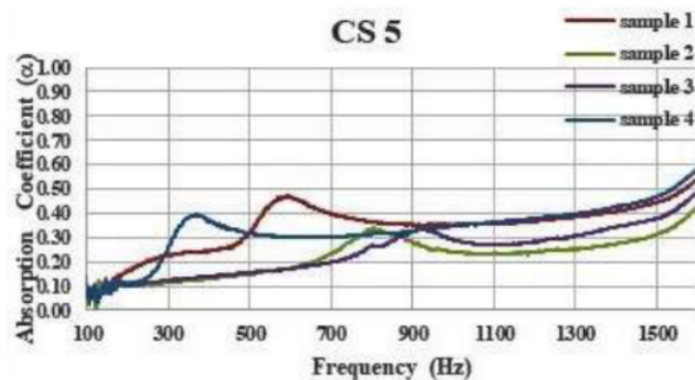
Figure 10 Absorption coefficient of CS5
