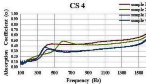
Figure 8 Absorption coefficient of CS4
