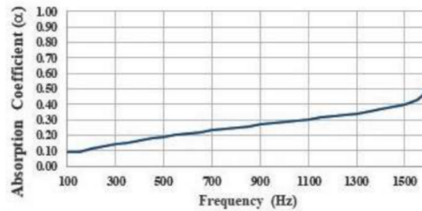
Figure 7. Average absorption coefficients of Flat Surface (FS) specimen
