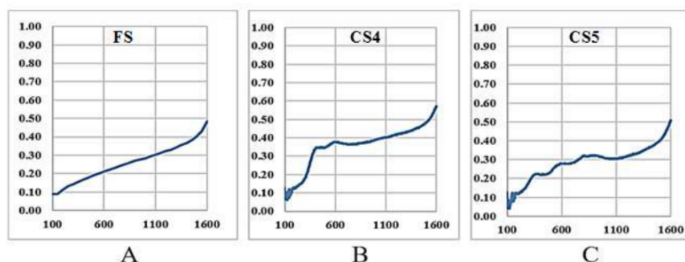
Figure 12. Average absorption coefficients of: A) FS sample; B) CS4 sample; C) CS5 sample.
