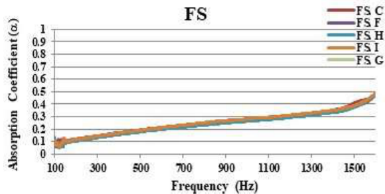
Figure 6. FS Absorption Coefficient Curve (C-F-H-I-G) sample
