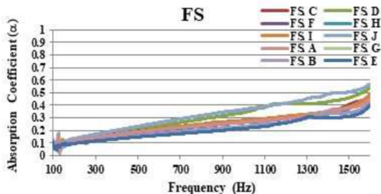
Figure 5. Absorption Coefficient of FS (A-J) samples
