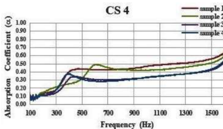
Figure 8 Absorption coefficient of CS4
