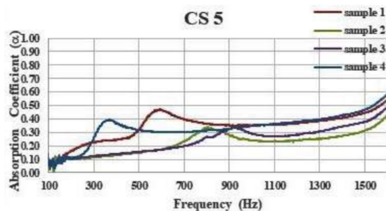
Figure 10 Absorption coefficient of CS5
