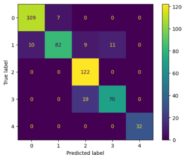
Figure 3: Confusion Matrix
