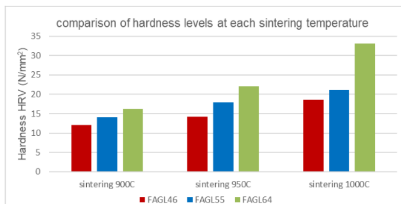
Figure 8. Average level of hardness on different sintering temperature
