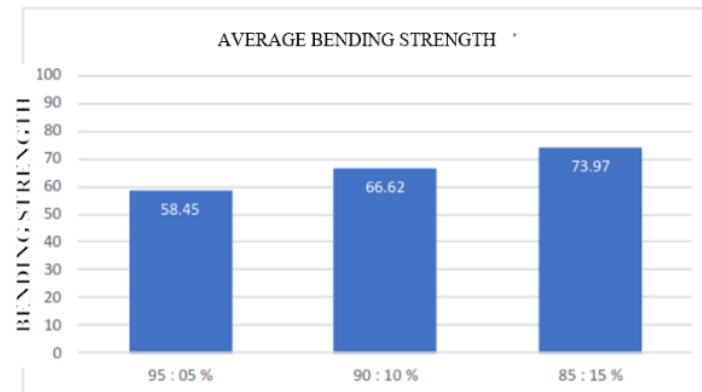
Figure 4. Average Bending strength for each weight fraction
