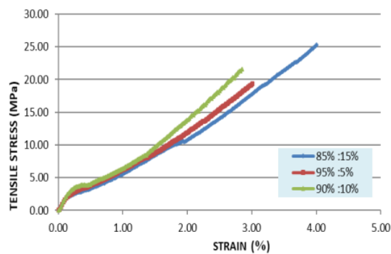
Fig. 3. Tensile Test results
