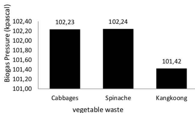
FIGURE 3. Optimal biogas pressures of various vegetable wastes
