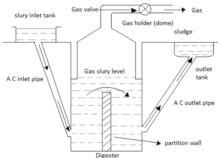
FIGURE 1: A set of biodigester
