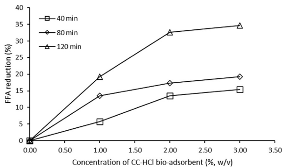
Figure 3. The effect of CC-HCl bioadsorbent concentration on FFA reduction.
