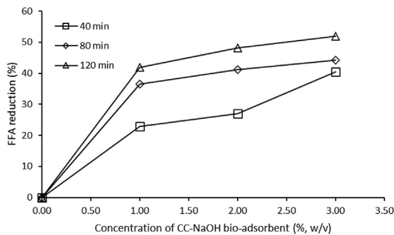
Figure 4. The effect of CC-NaOH bioadsorbent concentration on FFA reduction.
