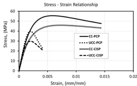
Fig. 5 Concrete stress-strain relationship
