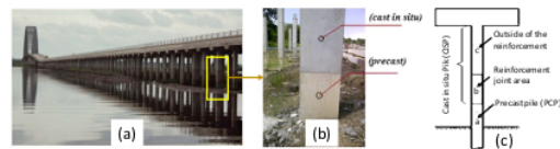
Fig. 1 Study site in (a) Bridge Column in Kutai Kertanegara Regency, East Kalimantan, (b) precast and cast in situ position, (c) diagram of column structure
