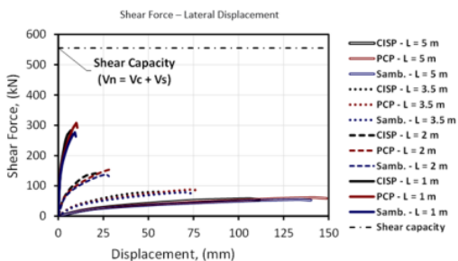
Fig. 8 Pillar lateral force-displacement relationship
