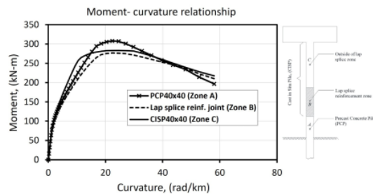
Fig. 6 Moment-curvature relationship of pillar cross-section
