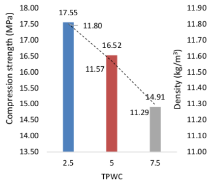
Fig. 9 Compressive strength - density
