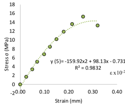
Fig.11 Modulus elasticity of TPWC 5
