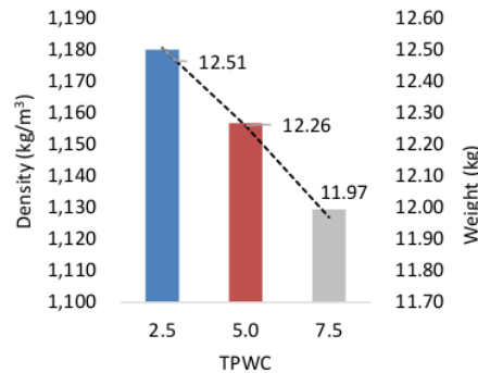
Fig.6 Density – weight
