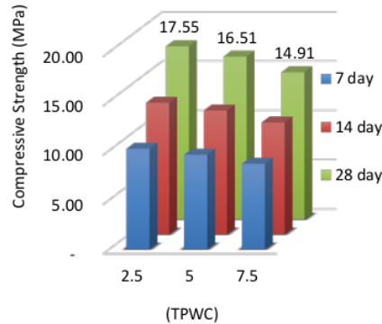
Fig.8 Compressive strength development of TPWC
