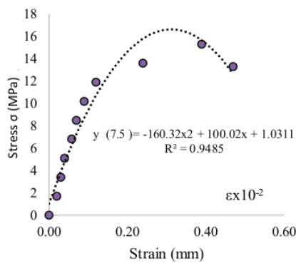
Fig 12 Modulus elasticity of TPWC 7.5
