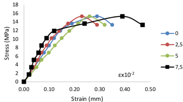
Fig.14 Stress-strain of TPWC
