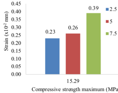
Fig.13 Compressive strength maximum - strain
