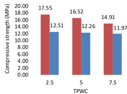
Fig.7 Compressive strength – weight
