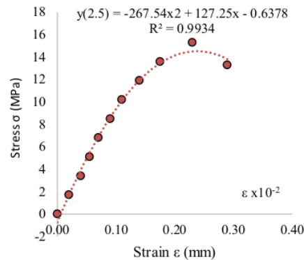
Fig.10 Modulus elasticity of TPWC 2.5
