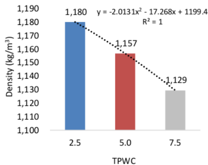
Fig 5. Density results
