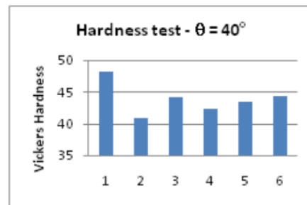
Fig 6: Hardness test results for a 40° spray angle
