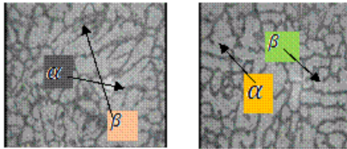
Fig.1: 400X microstructure phase
