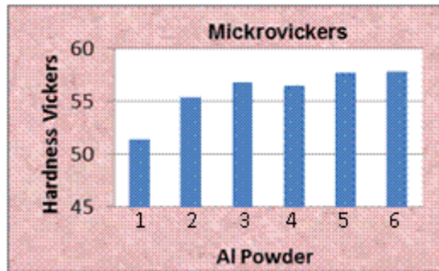
Fig. 6: L20° 8 mesh screen Hardness Test Results
