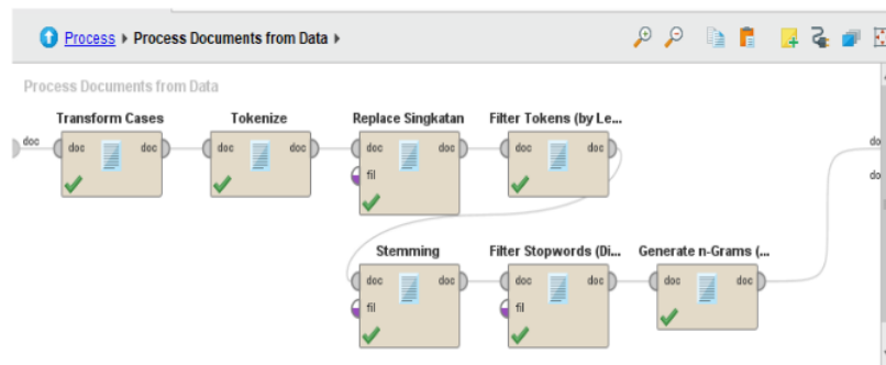
Figure 2. Preprocessing
