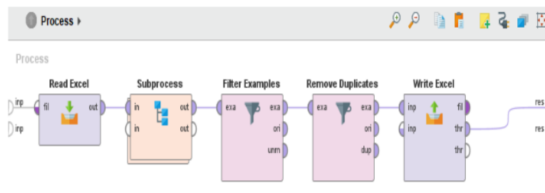
Figure 1. Data Cleaning
