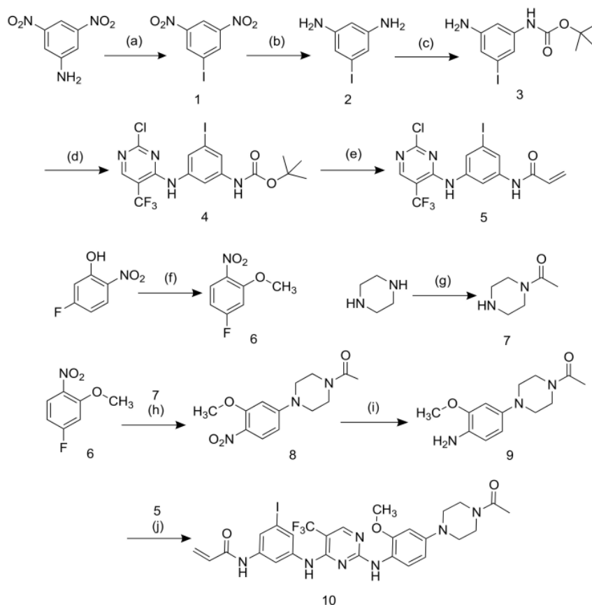
Scheme 1. Synthetic scheme of non-radioactive iodinated compound. Reagent: (a) \text{H}_2\text{SO}_4 , \text{NaNO}_2 , KI, 0^\circ\text{C} , rt, 3 h; (b) Ethanol, \text{SnCl}_2 \cdot 2\text{H}_2\text{O} , 45^\circ\text{C} , 1 h; (c) Acetonitrile, \text{Boc}_2\text{O} , rt, 2 h; (d) n -butanol, 2,4-dichloro-5-(trifluoromethyl) pyrimidine, DIPEA, 0^\circ\text{C} , 1 h, rt, 4 h; (e) HCl/ethyl acetate, rt, 1 h, dichloromethane, acryloyl chloride, DIPEA, -30^\circ\text{C} , rt, 1 h; (f) Acetone, \text{K}_2\text{CO}_3 , \text{CH}_3\text{I} , 0^\circ\text{C} , 5 h; (g) Dichloromethane, acetic anhydride, 0^\circ\text{C} , 5 h; (h) DMA, DIPEA, 90^\circ\text{C} , overnight; (i) Pd/C 10%, \text{H}_2 , rt, 5 h; (j) Dioxane, TFA, 60^\circ\text{C} , 3 h.
