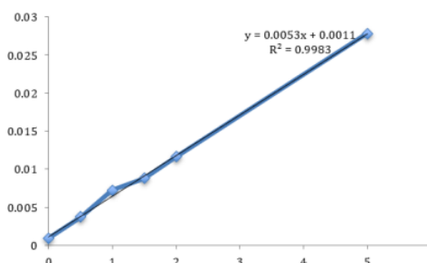
Figure 2. Calibration curve of lead (Pb)
