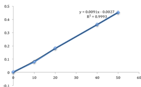
Figure 1. Calibration curve of mercury (Hg)
