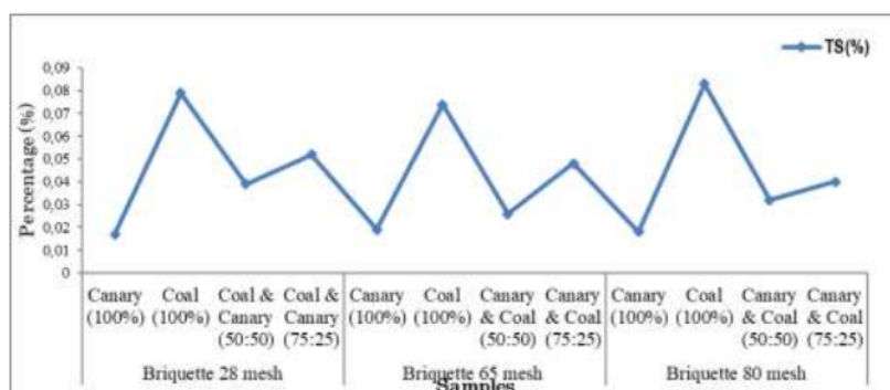
Figure 4. Effect of the briquetting on the sulfur content.
