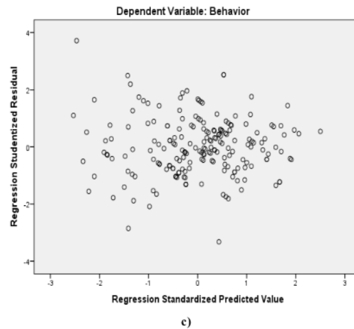
Figure 1. Classic Assumption Test; a) Residual Normality Histogram; b) P-P Plot Regression Standardized Residual Normality; and c) Scatter Plot Heteroscedasticity
