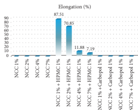
FIGURE 6: The elongation (%) values for 1%, 2%, 4%, and 7% NCC with hydroxypropyl methylcellulose (HPMC) and carbopol.
