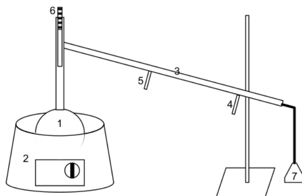
FIGURE 1. Distillation apparatus.
