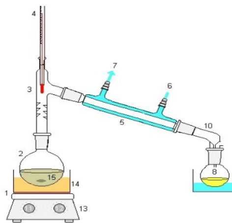
Fig. 1. Distillation apparatus
