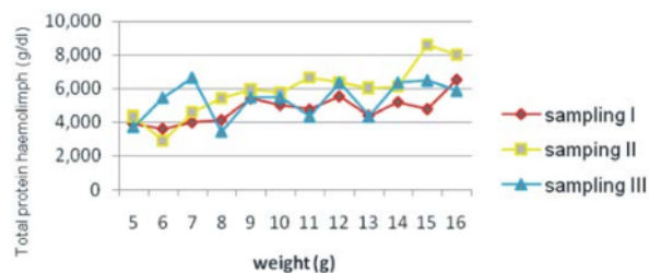
Fig. 2: Graph relationship between weights (g) of juvenile tiger prawn with total protein haemolymph (g/dl)
