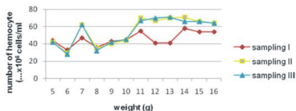
Fig. 1: The relationship between the weight (g) of juvenile tiger prawn against the number of hemocytes
