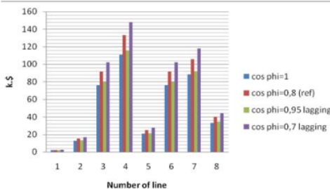
Fig. 5. The relationship between total costs ( C_k, F_k, L_k ) of the power factor in each line that contribute to the load #3
