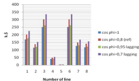
Fig. 3. The relationship between total costs ( C_k, F_k, L_k ) of the power factor on each line that contribute to the load # 1
