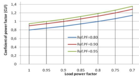
Fig.1 Coefficient power factor base on reference
