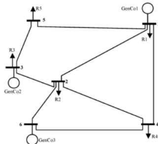
Fig. 2. Bus test Graver's
