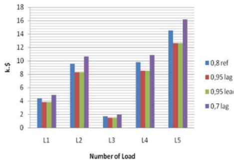
Fig. 7. The relationship between total costs ( C_k.F_k.L_k ) of the power factor in each line that contribute to the load #5
