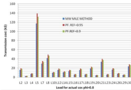
Fig. 8. Transmission cost of each load with actual power factor of 0.8
