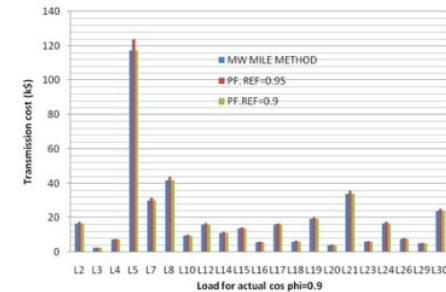
Figure 9. Transmission cost of each load with actual power factor of 0.9.
