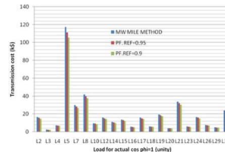
Fig. 10. Transmission cost of each load with actual power factor of unity
