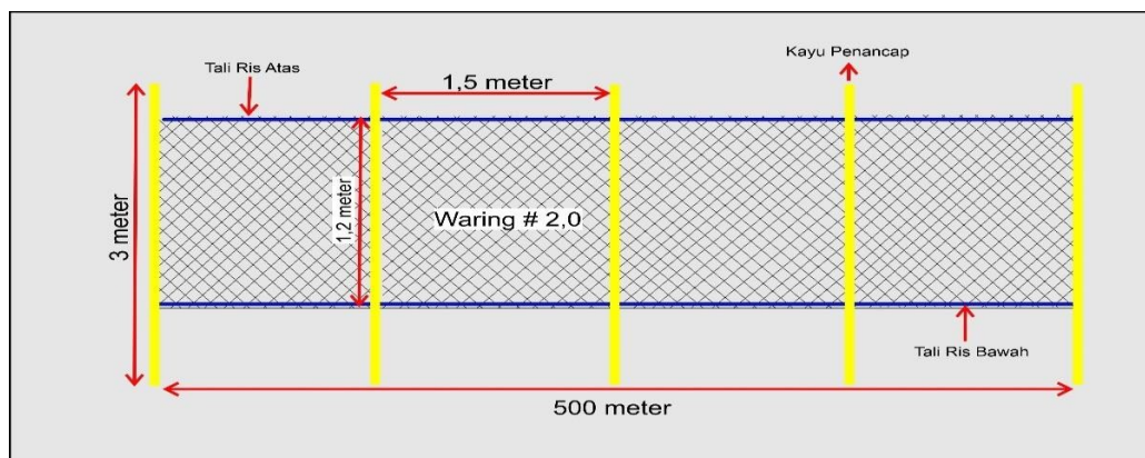
Figure 1. Description of the trap net
