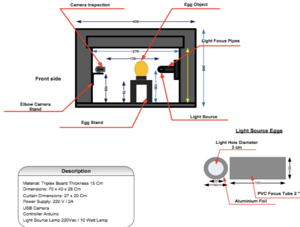
Fig. 1. Design Feature of an Egg Detection Box
