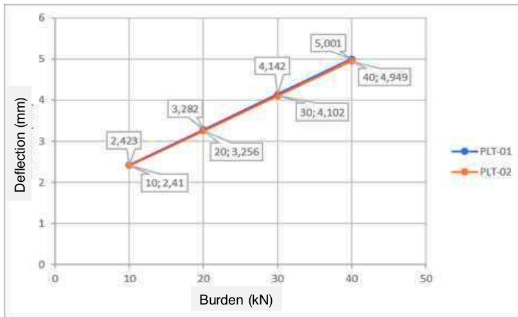
Figure 5. Relationship between burden (load) and deflection
