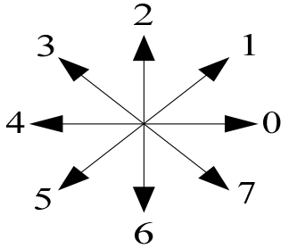
Fig. 2 Chain code
