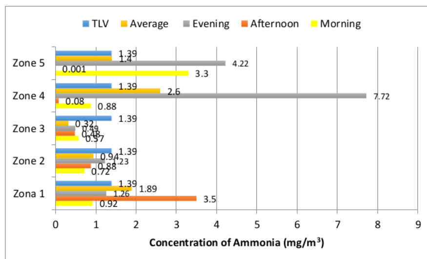
Graph 1. Comparison of Ammonia ( \text{NH}_3 ) Measurement Results in TPA Tamangapa with Threshold Limit Value (TLV)
