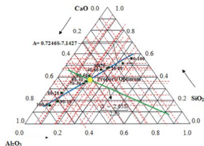
Fig. 6: Intersection point between mixing line with balance line
