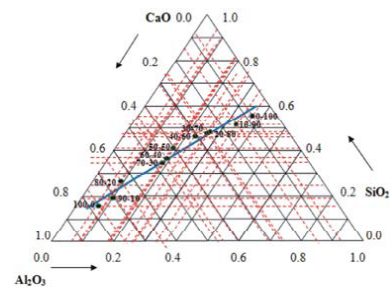
Fig. 4: Lines coordinate of cement + fly ash mix
