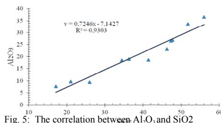
Fig. 5: The correlation between Al_2O_3 and SiO_2
