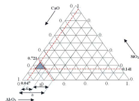
Fig. 2: The position between (0-100) on system ternary phase's diagram
