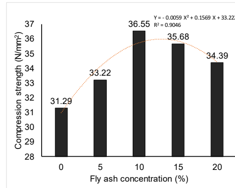
Figure 2. Optimum fly ash concentration for the highest compression strength
