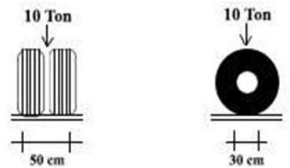
Fig 6: Loading System Due to Vehicle Loads
