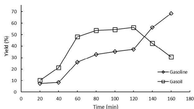
Figure 4. The product distribution of gasoline and gasoil as function of time at 350 °C and in the presence of CoMo/ \gamma -Al 2 O 3 catalyst
