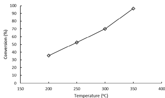
Figure 3. The effect of reaction temperature on conversion in the presence of \text{CoMo}/\gamma\text{-Al}_2\text{O}_3 catalyst
