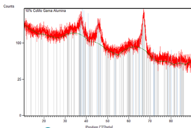
Figure 1. XRD patterns of \text{CoMo}/\gamma\text{-Al}_2\text{O}_3 catalyst
