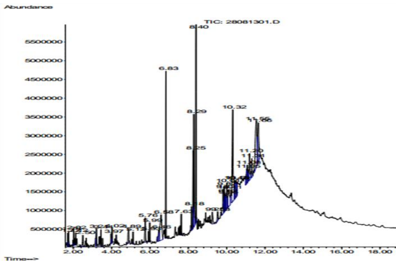
Figure 5. Chromatogram hydrocracking of CoMo/SiO 2 catalyst
