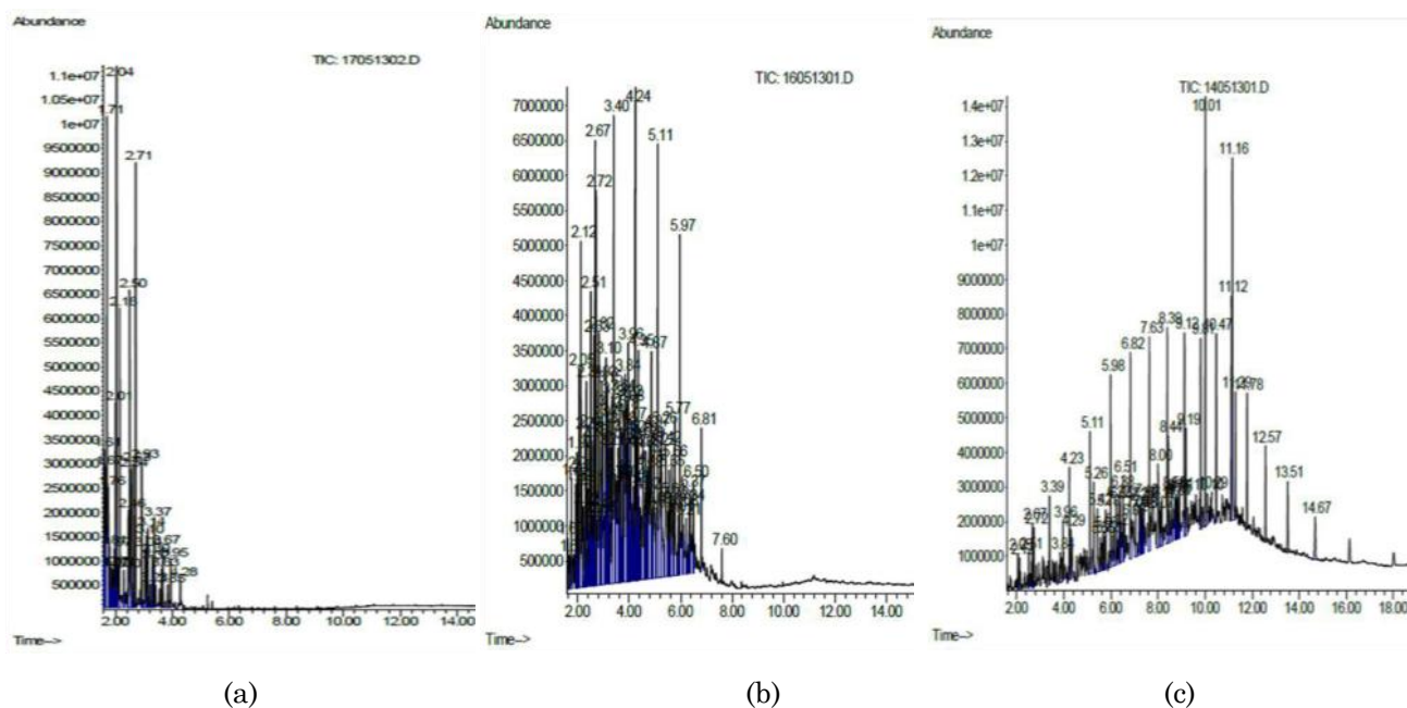
Figure 3. Chromatogram of GCMS for various commercial fuel: (a). Gasoline, (b). Kerosene, (c). Gasoil
