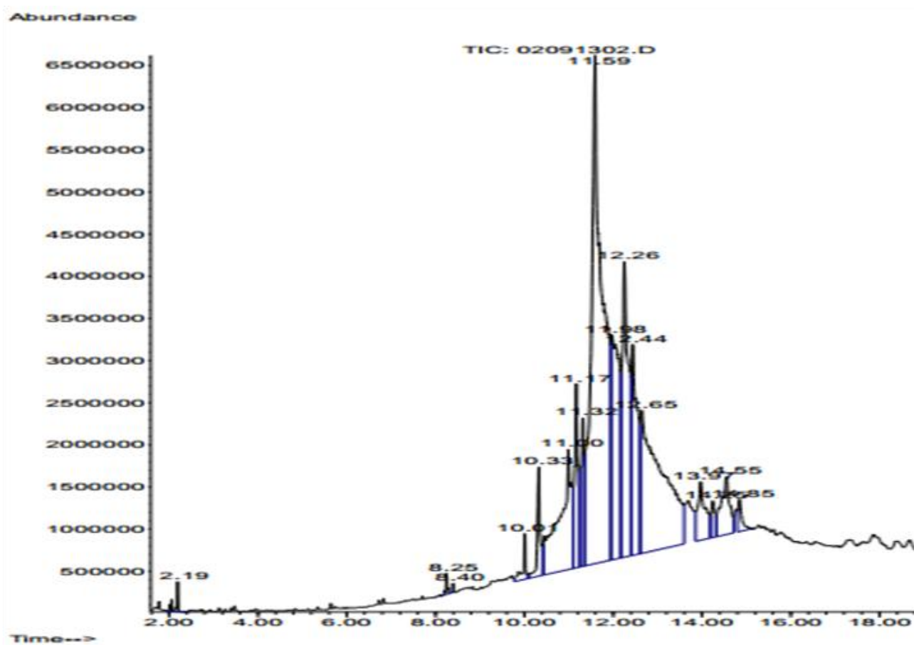
Figure 6. Chromatogram hydrocracking of CoMo/ \gamma -Al 2 O 3 -SiO 2 catalyst
