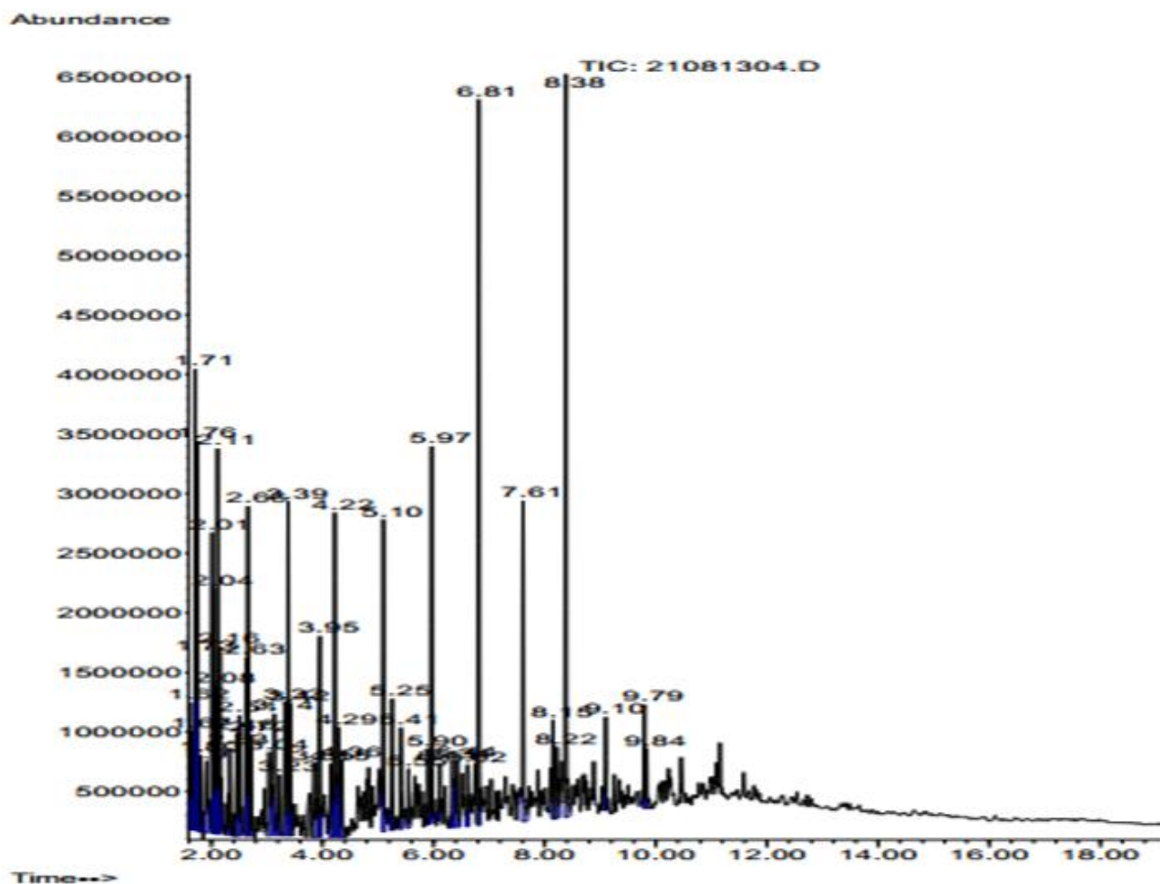
Figure 4. Chromatogram of hydrocracking product over catalyst of CoMo/ \gamma -Al 2 O 3
