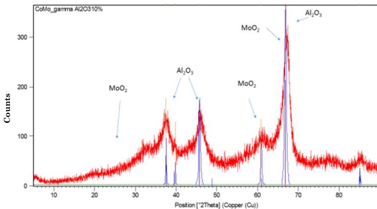
Figure 2. XRD of catalyst CoMo/gamma-Al 2 O 3
