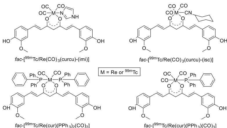
Figure 4. The chemical structure of \text{fac-}[^{99m}\text{Tc}/\text{Re}(\text{CO})_3(\text{curcu})-(\text{imi})] , \text{fac-}[^{99m}\text{Tc}/\text{Re}(\text{CO})_3(\text{curcu})-(\text{isc})] , \text{fac-}[^{99m}\text{Tc}/\text{Re}(\text{cur})-(\text{PPh}_3)_2(\text{CO})_2] , and \text{fac-}[^{99m}\text{Tc}/\text{Re}(\text{cur})-(\text{PPh}_3)(\text{CO})_3]
