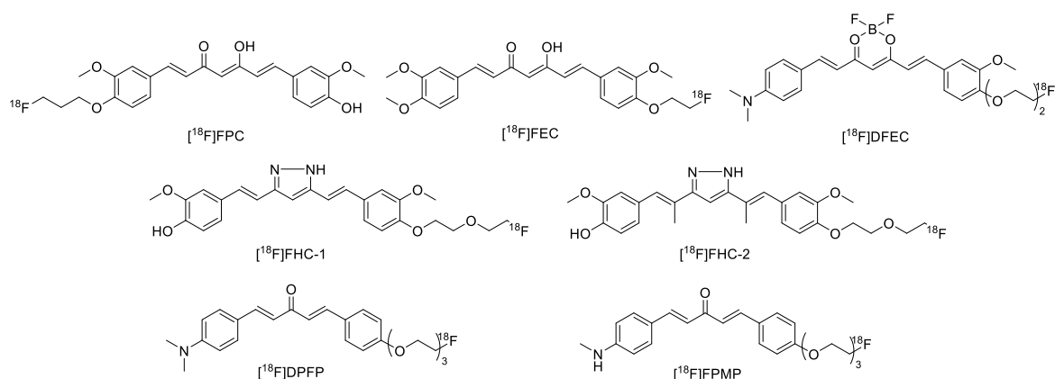
Figure 2. The chemical structure of [ 18 F]FPC, [ 18 F]FEC, [ 18 F]DFEC, [ 18 F]FHC-1, [ 18 F]FHC-2, [ 18 F]DPFP, and [ 18 F]FPMP
