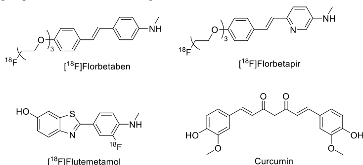
Figure 1. The chemical structure of [ ^{18}\text{F} ]florbetapir, [ ^{18}\text{F} ]florbetaben, [ ^{18}\text{F} ]flutemetamol, and curcumin
