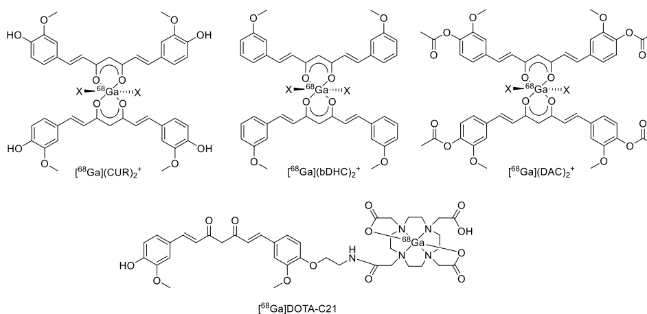
Figure 6. The chemical structure of [^{68}\text{Ga}](\text{CUR})_2^+ , [^{68}\text{Ga}](\text{bDHC})_2^+ , [^{68}\text{Ga}](\text{DAC})_2^+ , and [^{68}\text{Ga}]\text{DOTA-C21}
