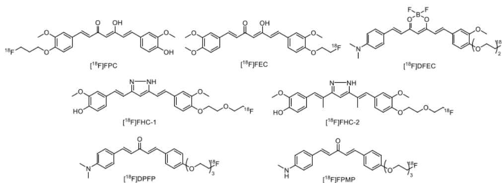
Figure 2. The chemical structure of [^{18}\text{F}]\text{FPC} , [^{18}\text{F}]\text{FEC} , [^{18}\text{F}]\text{DFEC} , [^{18}\text{F}]\text{FHC-1} , [^{18}\text{F}]\text{FHC-2} , [^{18}\text{F}]\text{DPFP} , and [^{18}\text{F}]\text{FPMP}
