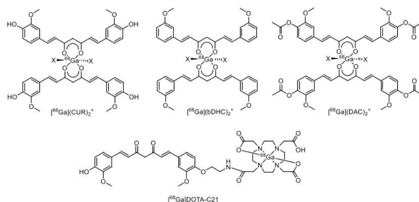
Figure 6. The chemical structure of [^{68}\text{Ga}](\text{CUR})_2^+ , [^{68}\text{Ga}](\text{bDHC})_2^+ , [^{68}\text{Ga}](\text{DAC})_2^+ , and [^{68}\text{Ga}]\text{DOTA-C21}
