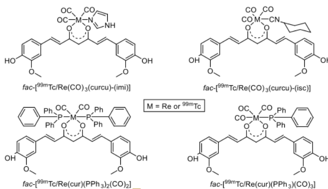
Figure 4. The chemical structure of fac -[ 99m Tc/Re(CO) 3 ( curcu )-(imi)], fac -[ 99m Tc/Re(CO) 3 ( curcu )-(isc)], fac -[ 99m Tc/Re( cur )-(PPh 3 ) 2 (CO) 2 ], and fac -[ 99m Tc/Re( cur )-(PPh 3 )(CO) 3 ]
