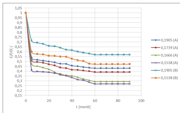
Figure 3. The ratio of the concentration of phenol compounds in residual solution of initial concentrations of phenol compounds against (C/C_0) as a function of time (t) on a variety of active carbon/mass ratio of the mass of the solution (r) .
