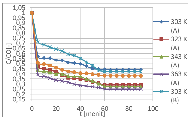
Figure 1. The ratio of the concentration of phenol compounds in residual solution of initial concentrations of phenol compounds against (C/C_0) as a function of time (t) on a wide range of operating temperatures (T) .
