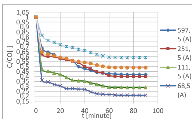
Figure 2 . The ratio of the concentration of phenol compounds in residual solution of initial concentrations of phenol compounds against (C/C_0) as a function of time (t) activated carbon range of grain size (d)
