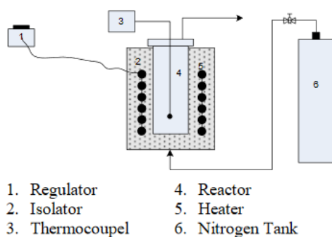
Figure 1. The schematic diagram of the pyrolysis apparatus.
