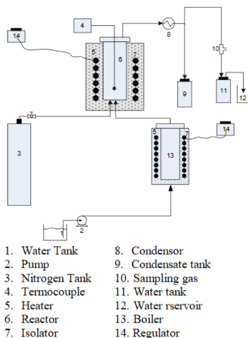
Figure 2. The schematic diagram of the gasification apparatus
