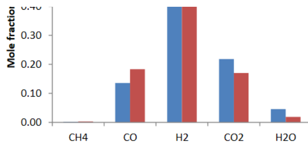
Fig. 6c. Comparison of mole fraction from thermodynamics model and experimental data at gasification temperature 800 °C for model 1
