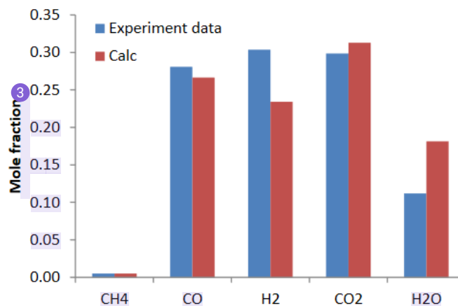
Fig. 7b. Comparison of mole fraction from thermodynamics model and experimental data at gasification temperature 700 °C for model 2.
