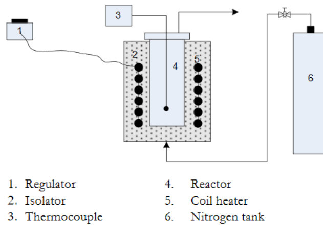
Fig. 2. The schematic diagram of the pyrolysis apparatus.
