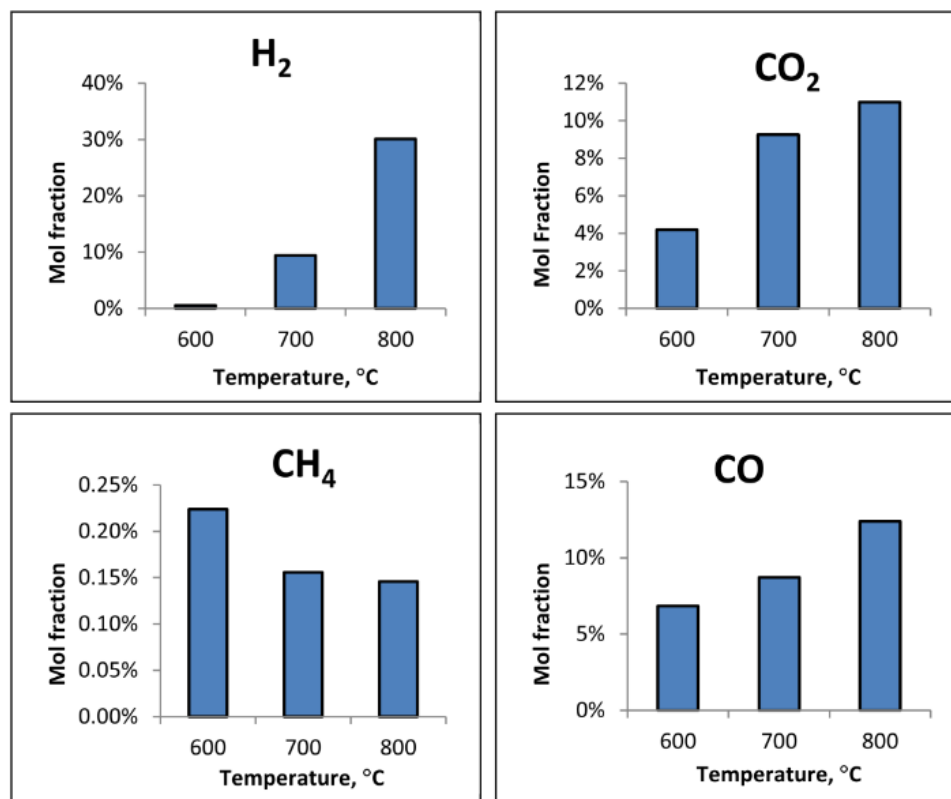
Fig. 5. Effect of temperature on the gas composition at 600, 700, and 800 °C for 60 minutes.
