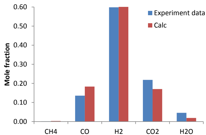
Fig. 6c. Comparison of mole fraction from thermodynamics model and experimental data at gasification temperature 800 °C for model 1
